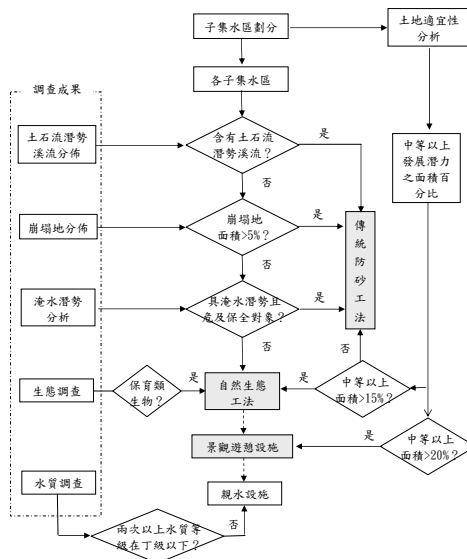
圖3. 北坑溪生態工法區位之規劃流程圖 Figure 3. Integrated treatments planning for Bei-Keng stream watershed.
