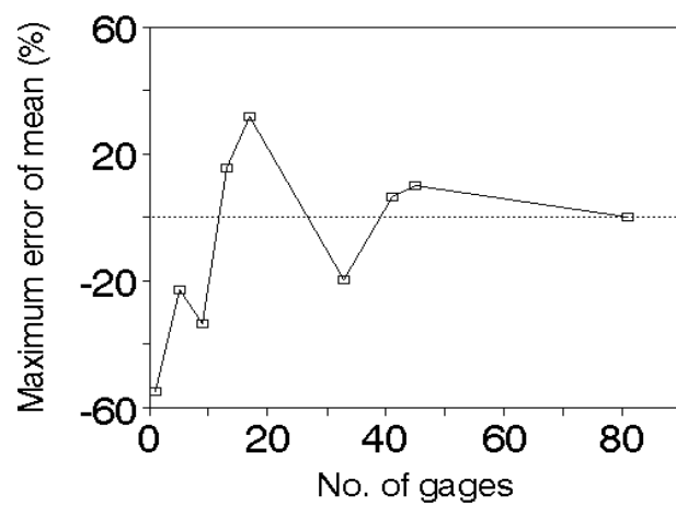
圖 6. 檳榔園 12 場不同數量量筒穿落雨的最大誤差率 Fig. 6. Maximum error of mean of measured throughfall in betel palm plantation under different number of gages for 12 events.
