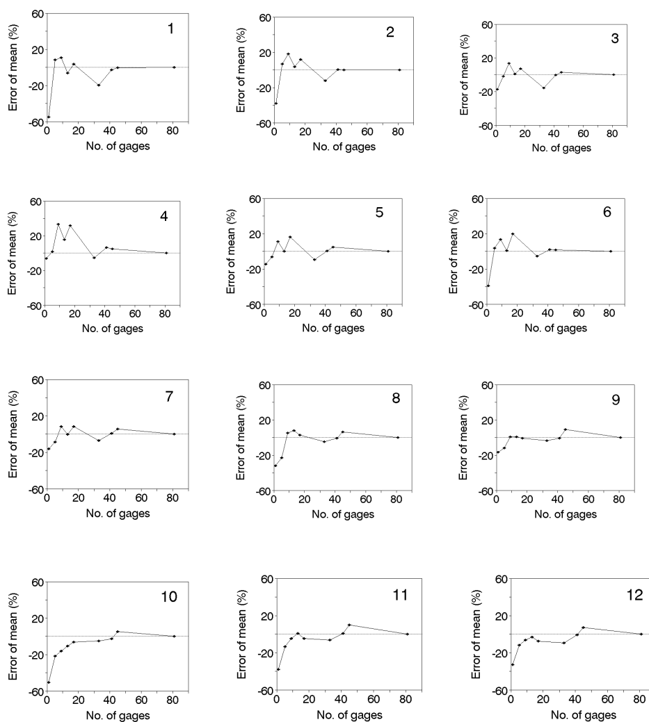
圖 3. 檳榔園不同數量量筒(20 公分直徑承雨口)計算 12 場穿落雨平均值之誤差率 Fig. 3. Error of mean of measured throughfall from different number of gages (20 cm in diameter) for 12 events at betel palm plantation.
