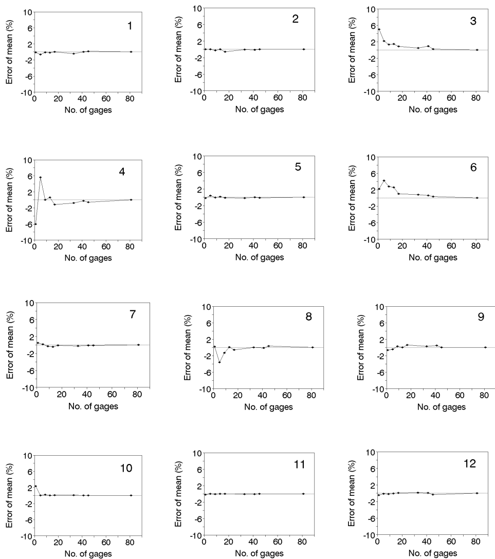
圖 4. 空曠地不同數量量筒(20 公分直徑承雨口)計算 12 場降雨平均值之誤差率 Fig. 4. Error of mean of measured rainfall from different number of gages (20 cm in diameter) for 12 events at bare land.
