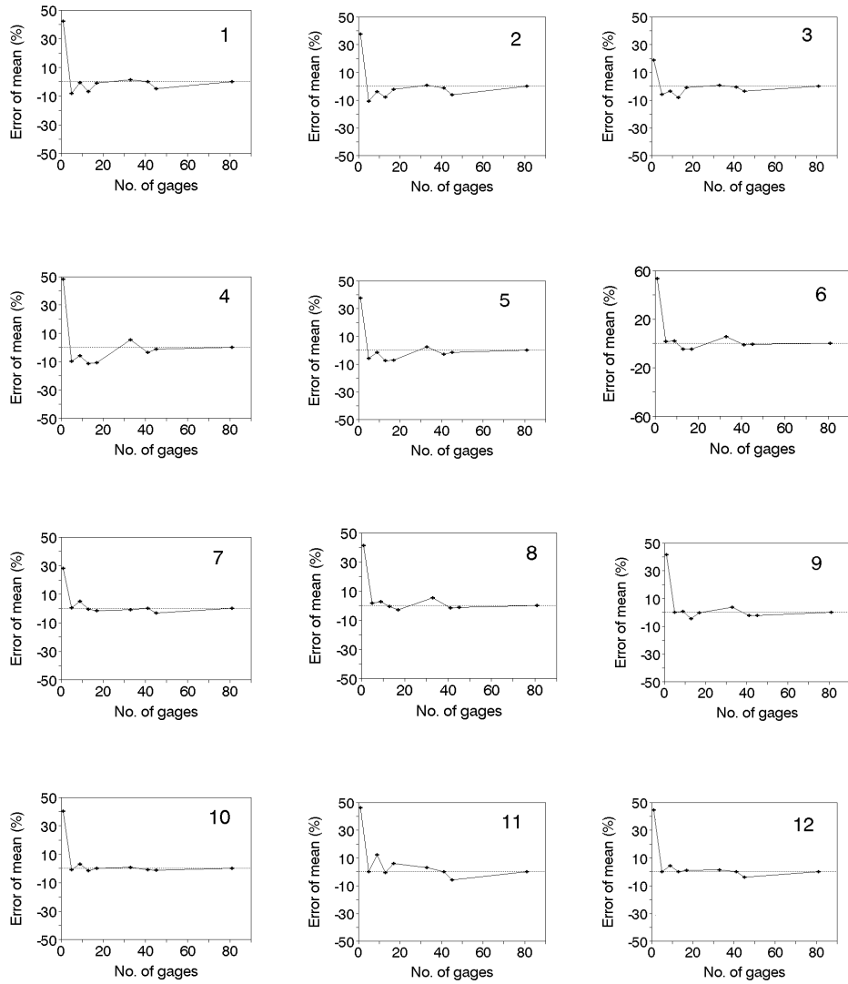
圖 2. 天然闊葉林不同數量量筒(20 公分直徑承雨口)計算 12 場穿落雨平均值之誤差率 Fig. 2. Error of mean of measured throughfall from different number of gages (20 cm in diameter) for 12 events at natural hardwood forest.
